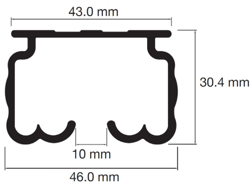
Track cross-section 1
